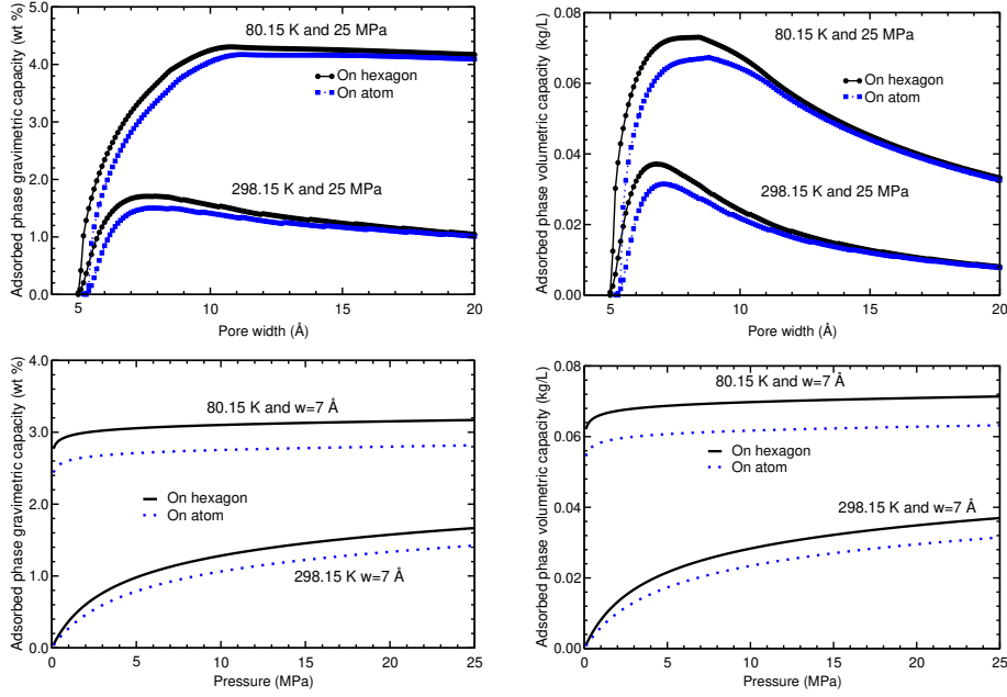
Fig. 5. Gravimetric and volumetric hydrogen storage capacities of graphene slit pores for 80.15 K and 298.15 K and two configurations, H_{\text{III}} and A_{\text{III}} . Upper panel: Capacities as functions of the pore width, for a pressure of 25 MPa. Lower panel: Capacities as functions of the pressure, for a pore width of 7 Å.
