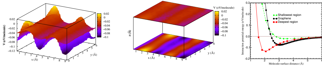
Fig. 2. Interaction potential energy between a single Li-decorated \beta borophene sheet and a H_2 molecule in the planes z = 2.58 and 3.33 \text{ \AA} plotted in 3D (left panel) and its projections in the xy plane (middle panel). The bottom and upper 3D surfaces (planes) of the left (middle) panel correspond to the planes z = 2.58 and 3.33 \text{ \AA} , respectively. Right panel: Interaction potential energy between a H_2 molecule and a single graphene layer, and a single Li-decorated \beta borophene sheet at the deepest and shallowest xy points, as a function of the H_2 molecule-surface distance.
