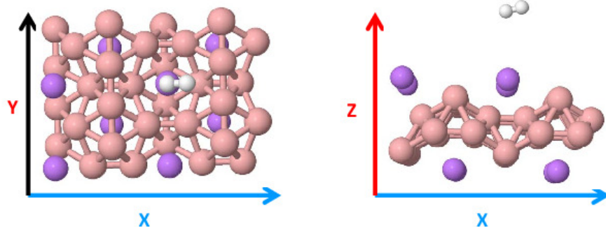
Fig. 1. Front and side views of the relaxed 2 \times 2 supercell of the \beta (Pmmn8) sheet decorated with 4 Li atoms at furrow sites on each side of the sheet. Li atoms are shown with purple balls. Also shown is an adsorbed \text{H}_2 molecule in its most stable configuration (with H atoms in white).
