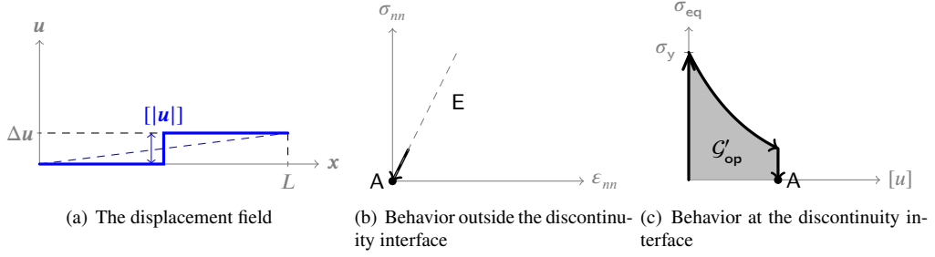
Figure 5: Local constitutive model at the continuous part and at the discontinuity interface as the imposed displacement decreases.
