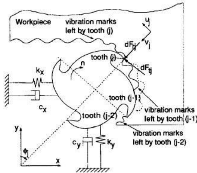
Figure 1. Milling model for two orthogonal degrees of freedom (Altintas, 2000).
