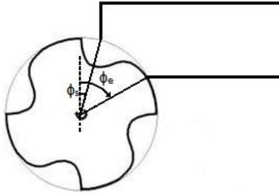
Figure 2. Entry and exit angles of the cut.
