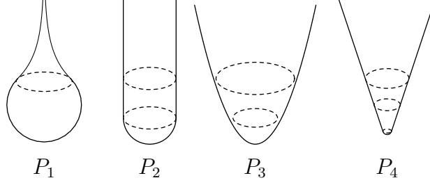
FIGURE 1. Sketch view of the four Riemannian planes of Example 2.6 with U(1) \rtimes \mathbf{Z}/2\mathbf{Z} symmetry.
