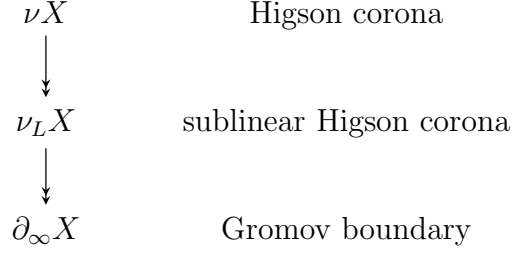
FIGURE 3. Coronae and Gromov boundary for hyperbolic X .
