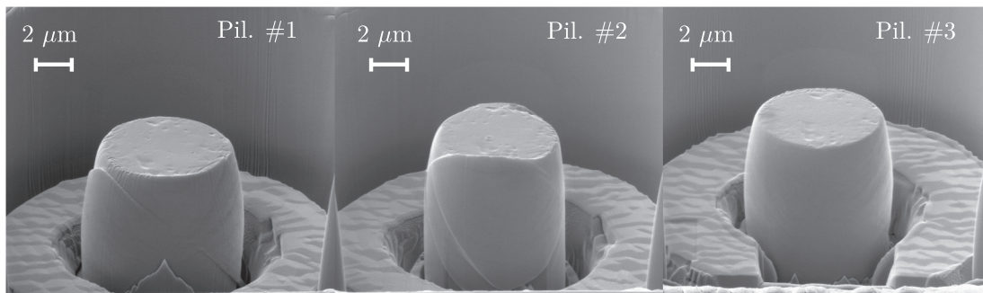
Fig. 7. 7 \mu\text{m} top diameter pillars deformed shapes after microcompression at \langle \dot{\epsilon} \rangle \approx 10^2 \text{ s}^{-1} . Pillars #1 and #2 both presented a clearly marked double-slip pattern. Pillar #3 presented a barrel shape with no sign of slip bands. The deformed pillar shapes explains the differences in the stress-strain curves observed in Fig. 5.
