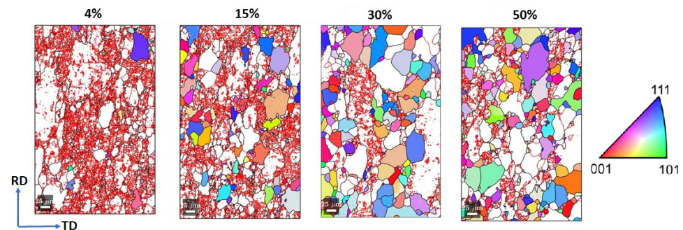
Figure 6. EBSD maps representing the evolution of softening fraction at T = 1550\text{ }^\circ\text{C} . The grain boundaries are in black, the sub-grain boundaries are in red and the recrystallized grains are colored according to (IPF Z—normal direction).
