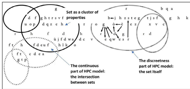
Figure 2. The HPC model as a Venn diagram. Letters are symptoms, arrows are symptom-symptom relationships (qualitatively pointing toward the right cluster only). Sets' boundaries bearing the same mark, represent the same disorder concept; smaller sets with the same mark represent the sub-cluster of that disorder (i.e., possible symptoms of patients). Sets with different marks represent different disorders. The continuous element of the HPC model is viewable as the intersection between sets; the discreteness of the HPC model is viewable as the sets themselves.
