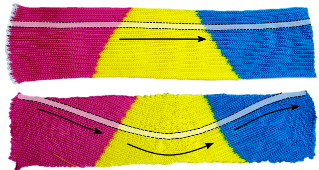
Fig. 12. The same rectangular shape with a 3-color texture was knitted with our system using an horizontally aligned (top) and an adaptive (bottom) vector field. In the latter, the color change only happens across courses and not within a course (Size: 200 x 50 mm).
