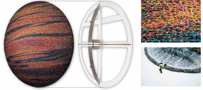
Fig. 18. A complex knitted object showcasing high-level capabilities of the KnitKit system. Custom 5-color stitch templates, action definitions for an integrated drawstring channel and shaping techniques are used to generate the object from a geometric and image texture input. Inset photos show the close-up details of the complex stitch pattern and drawstring channel.
