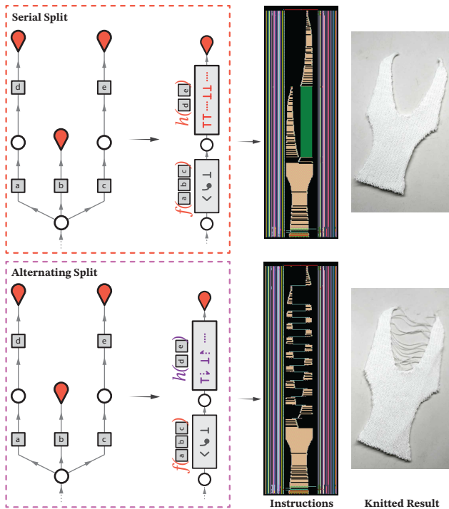
Fig. 15. Just by changing the split action rule, it is possible to generate instructions that use different scheduling strategies for dealing with split branches from the same KnitNet . The bottom strategy achieves more uniform tension by means of a single yarn carrier knitting both branches in an alternating manner with floating yarns as bridges.
