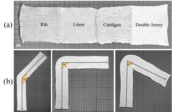
Fig. 11. The geometric calibration allows us to locally configure the parameterization process such that the resulting shape and size of the knitted output is in accordance with the geometric dimensions of the input design.
