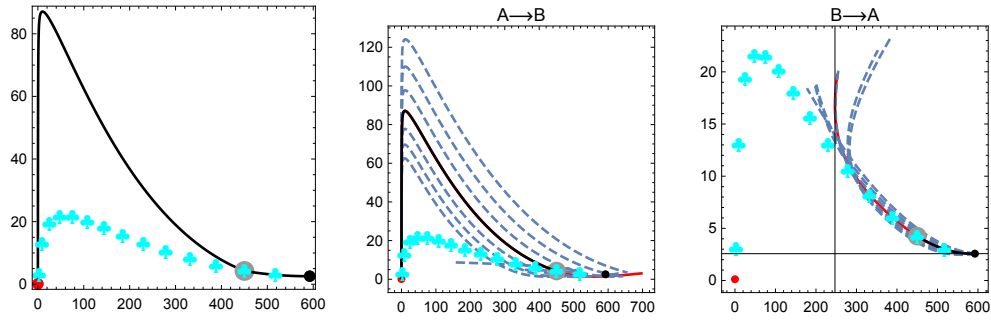
Figure S3: A numerical cut point with an unsatisfactory \widetilde{\gamma}_R . Same structure as S1. \{0.00996246, 0.121282\} \leftrightarrow \{592.392, 2.57454\} ; D_R = 43.1519
