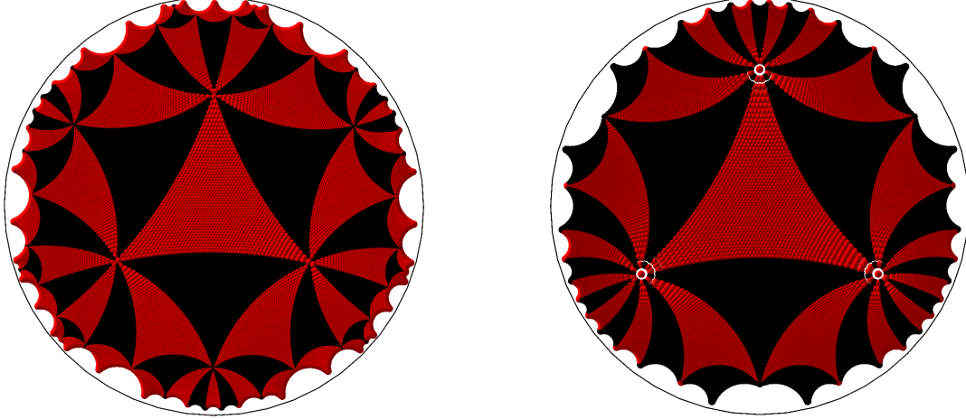
(A) The \{3, 10\} -tessellation of \Sigma(\widehat{I_2(5)}) \simeq \mathbb{H}^2 .
