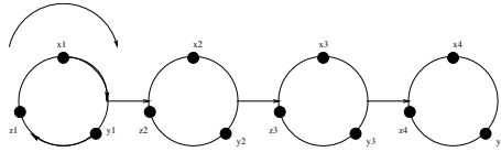
FIGURE 2. C_{3,4}
