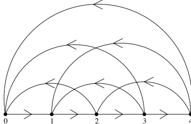
FIGURE 1. Path of strong connectivity on 5 vertices
