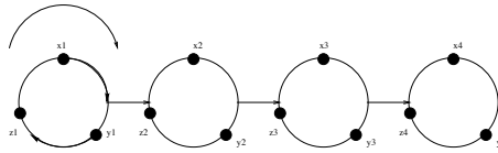
FIGURE 2. C_{3,4}
