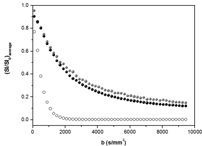
Figure 2. d MRI signal decay of RH (black symbols) and LH (gray symbols) averaged over the three orthogonal directions; for comparison, the averaged signal decay of free water (deionized water Milli-Q, open symbols) is also shown.
