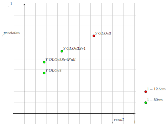
Fig. 2. Detection performance on the VEDAI data using the YOLOv3 detector associated with SR by a factor of 4. VEDAI images with different resolutions: red for 12.5cm/pixel and green for 50cm/pixel. Here, YOLOv3 is combined with SR trained on full images ( YOLOv3Sr4Full ) and SR focused on target objects ( YOLOv3Sr4 ).
