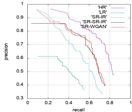
Fig. 5. Detection performance using object-focused super-resolution by SR-IR and SR-WGAN jointly with the Faster-RCNN detector (VEDAI dataset).
