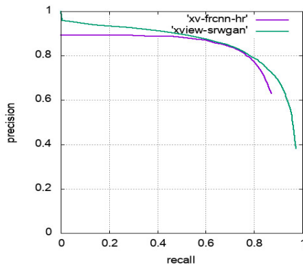
Fig. 7. Detection performance using Faster-RCNN detector on both standard and super-resolved images using SR-WGAN (xView dataset).
