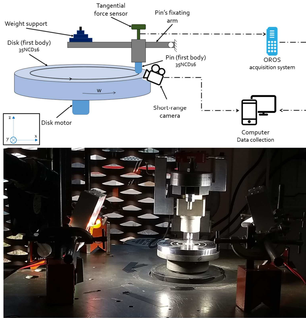
Fig. 1. Experimental apparatus
