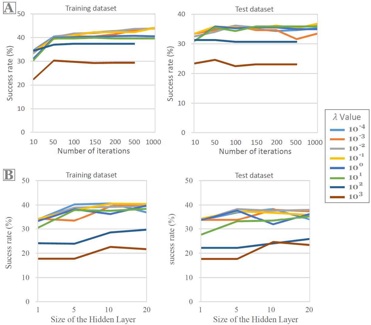
Fig. 6. Success rates of the classification algorithms. A. Logistic regression; B. Artificial Neural Network
