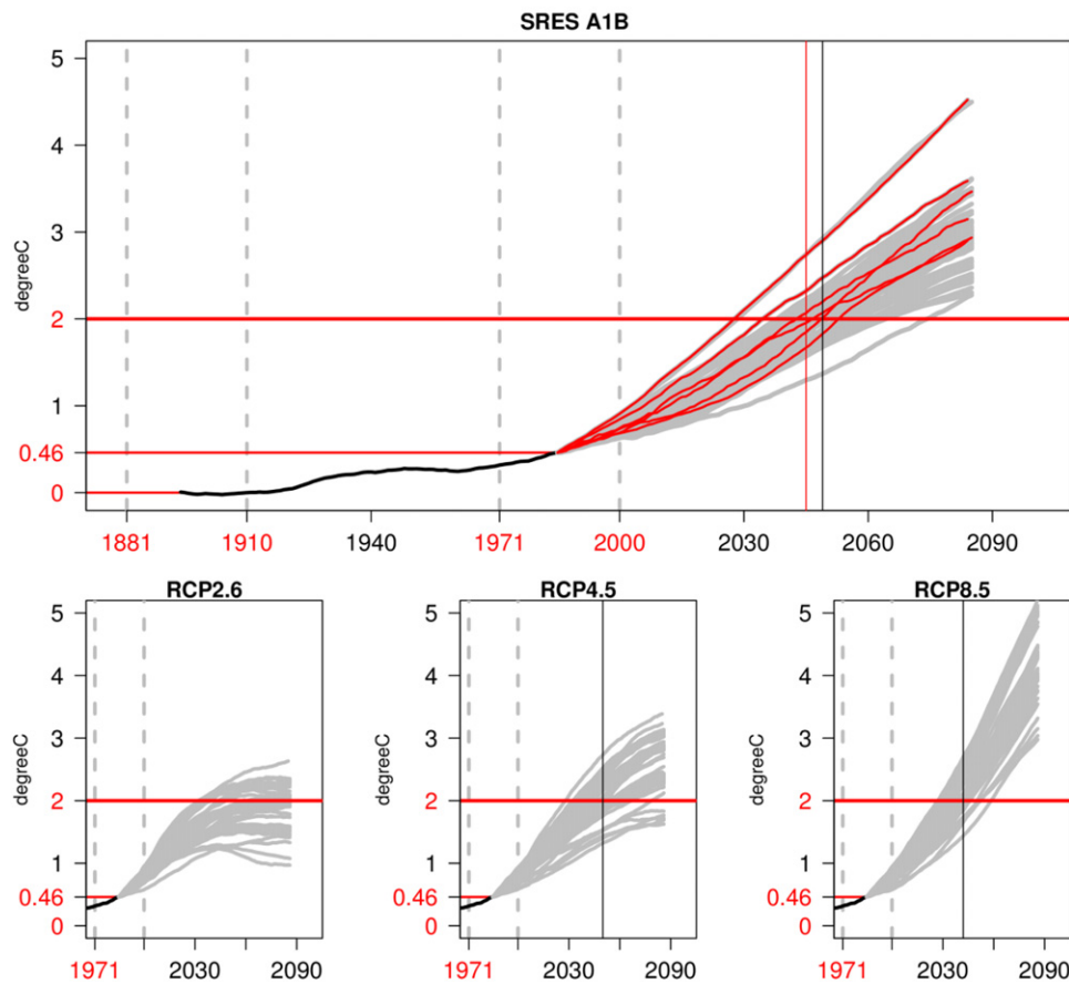
Figure 1. Global mean temperature (30-year running mean; gray lines) for the SRES A1B ensemble (top panel) and for the RCP2.6, RCP4.5 and RCP8.5 CMIP5 simulations (bottom panels) exceeding the +2 °C threshold (bold red horizontal line). The average observed temperature compared to pre-industrial (1881–1910) is depicted in the upper panel as black line. The CMIP3 and CMIP5 ensemble median years of reaching the 2 °C target for each emission scenario are shown as black vertical lines, whereas the red vertical line represents the median year of the six driving GCMs of this study, which are highlighted in red. Since most RCP2.6 simulations stabilize below +2 °C, no median exceedance year is shown.
