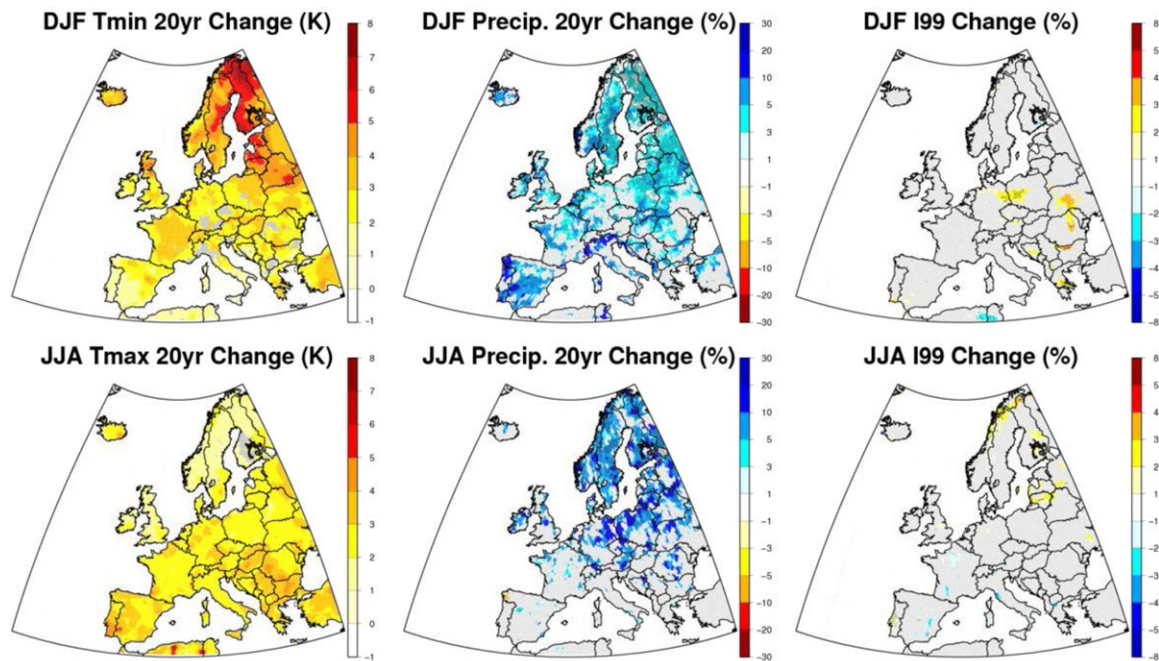
Figure 4. Changes, between the 1971–2000 and the +2 °C periods, in the 20-year return value for Tmin in winter (upper left), Tmax in summer (lower left), heavy precipitation in winter (top middle) and in summer (bottom middle), extreme winds (I99) in winter (top right) and in summer (bottom right). Only areas with at least 12 models agreeing on change sign are colored. Areas where at least 14 models agree on change sign are highlighted with dots (except for temperature where almost all areas satisfy this).
