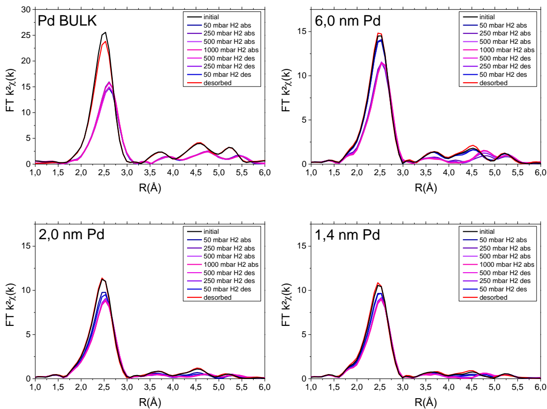
Figure 3. FT of the EXAFS spectra ( k^2 \chi(k) ) for bulk Pd and 6.0, 2.0 and 1.4nm Pd nanoparticles under various partial pressures of H_2 at 25 °C.
