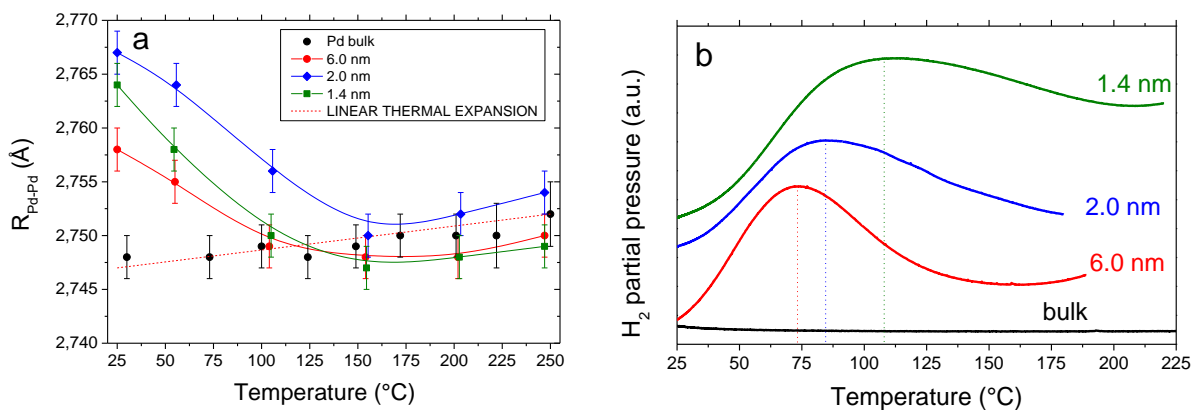
Figure 5. The thermal variation of R_{Pd-Pd} (A) and the TDS spectra (B) for bulk, 6.0, 2.0 and 1.4 nm Pd nanoparticles. In figure A, the expected linear thermal expansion of bulk Pd is also plotted.
