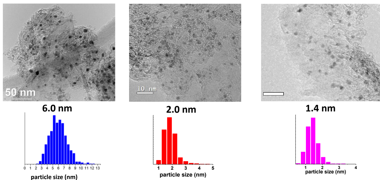
Figure 1. TEM images and related particle size histograms for 6.0 nm, 2.0 nm and 1.4 nm Pd nanoparticles supported on carbon.
