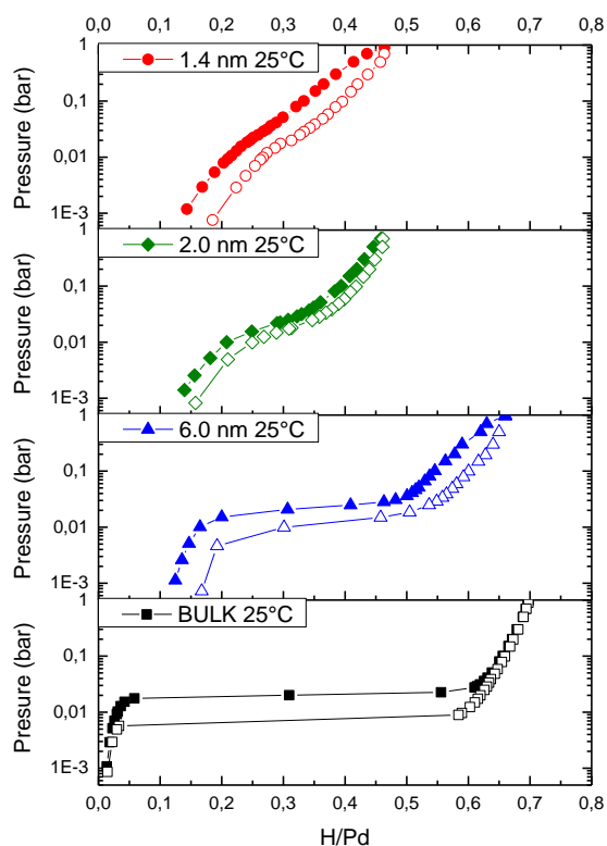
Figure 2. Pressure-composition-isotherms for bulk Pd (square) and Pd nanoparticles with average sizes of 6.0 nm (triangle), 2.0 nm (rhombus) and 1.4 nm (circle) at 25 °C. Full and empty symbols stand for absorption and desorption, respectively.
