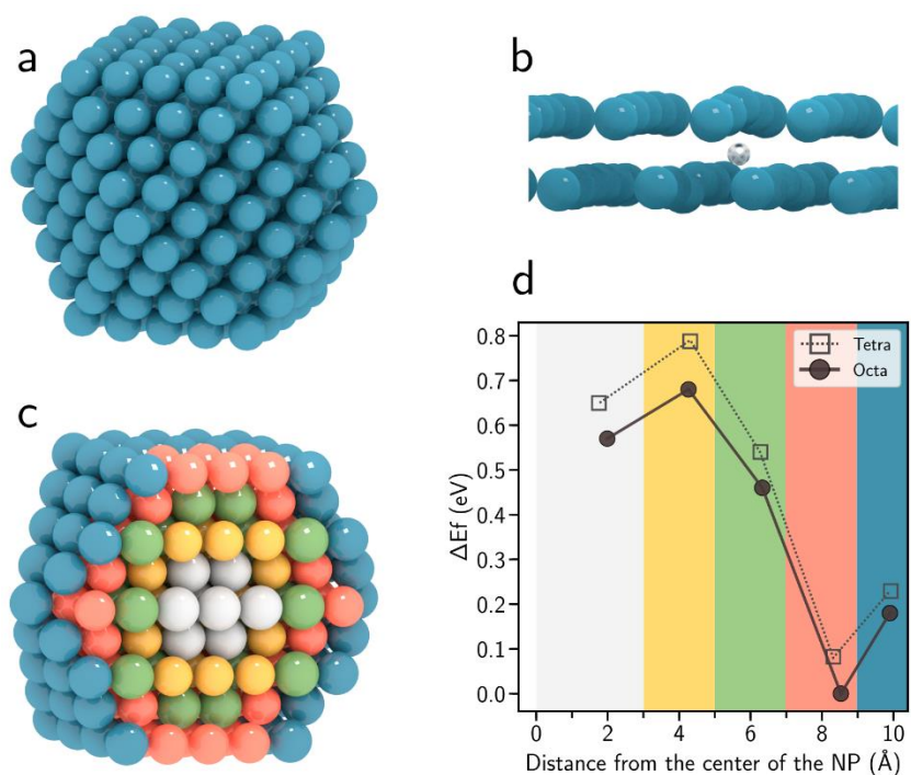
Figure 6. (a) Cuboctahedron NP of Pd containing 309 atoms. (b) Presence of the hydrogen atom (white) in the subsurface position of the NP inducing a local distortion of the first layers. (c) Slide view showing the different planes within the NP. (d) Formation energy of a hydrogen atom occupying different sites (octahedral and tetrahedral) along the radius of the NP. The different coloured areas correspond to the regions indicated in (c) : blue and red correspond to the surface and subsurface, respectively. The most stable configuration is set to zero.
