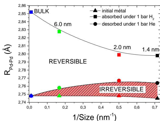
Figure 4. The variation of R_{Pd-Pd} as function of the inverse of particle size for several sizes of bulk Pd and nanoparticles as initial metal (triangle), hydride (square) and desorbed phase (circle).
