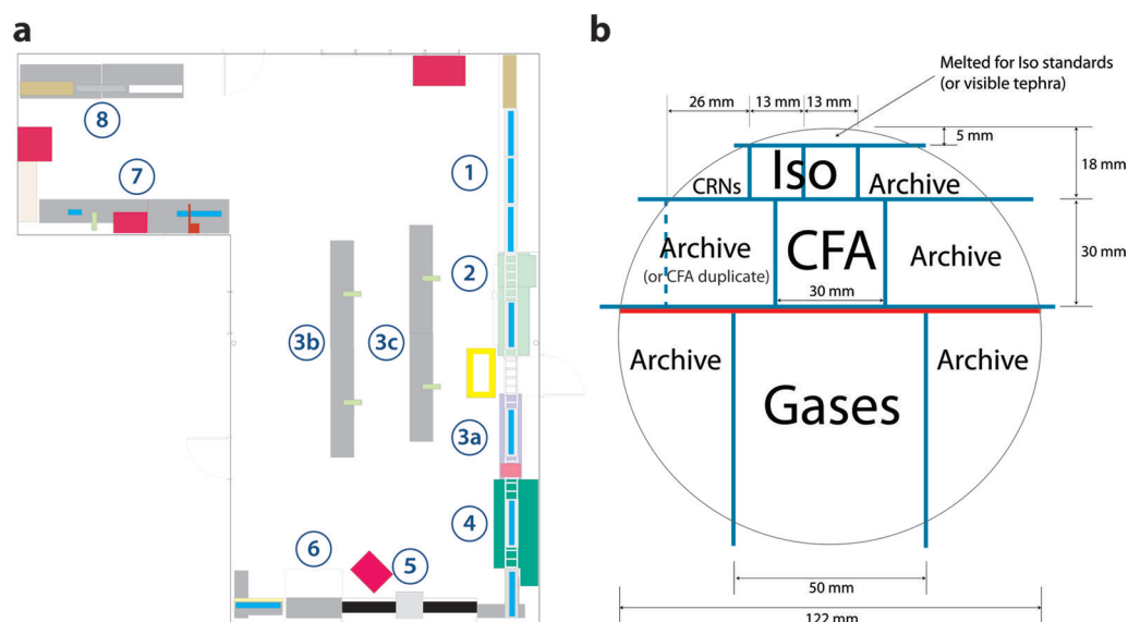
Fig. 12. (a) Generalized layout of the NICL's -24^{\circ}\text{C} exam room during the CPLs to process and sample ice from \sim 1300 to 3405 m. The circled numbers correspond to the circled numbers in the CPL flow chart (Fig. 13). The purple rectangles are logging computers. (b) Cross section of the ice core showing the generalized cut plan used from \sim 1300 to 3405 m. The thick red line represents the ice removed by the planer before the electrical properties are measured on the bottom half of the core. Iso = water stable isotopes; CFA = continuous flow analysis; CRNs = cosmogenic radionuclides. From 114 to 577 m depth, three 30 mm \times 30 mm CFA sticks were cut from the top half of the core.
