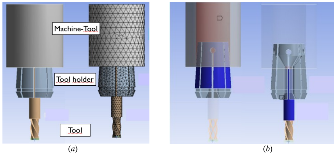
Figure 3. Tool Holder Assembly: (a) solid model and (b) finite element mesh. Numerical model.
