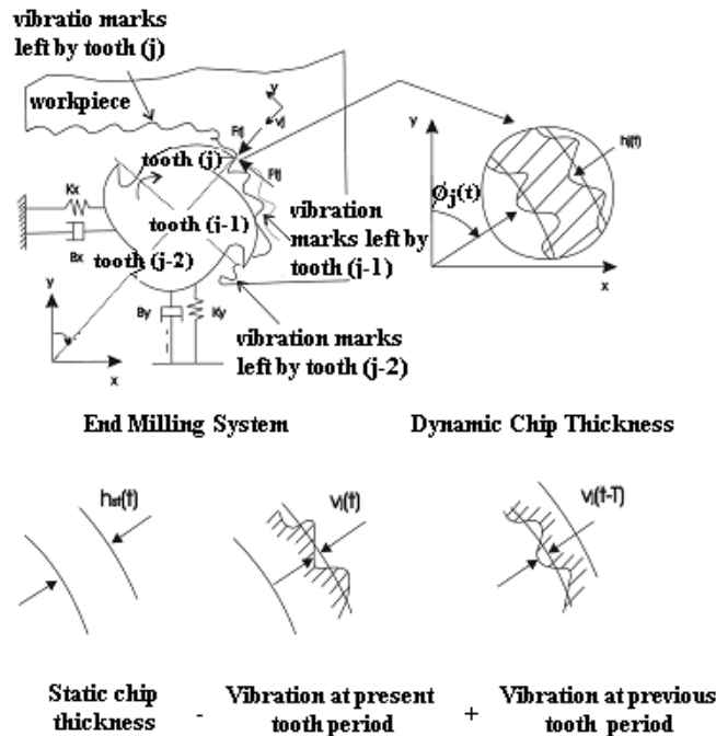
Figure 1. 2 DOF Dynamics of chatter on End Milling (Altintas, 2000)
