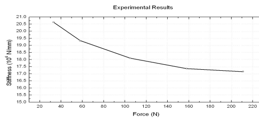
Figure 13. Stiffness as a function of the Applied Force
