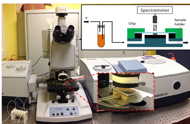
Figure 2: Experimental setup for microscale analysis and fluid-managing system used for optical detection.
