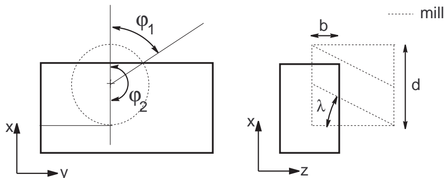
Figure 1. Milling geometry
