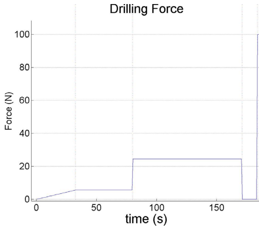
Figure 7. Drilling Force.
