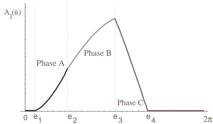
Figure 4. Area Function for one Single Flute.
