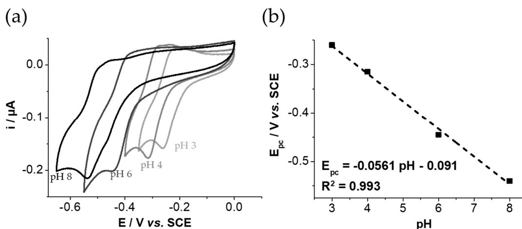
Figure 6. Electrochemical behavior of GNP PSCD solution ( 0.14 \text{ mg mL}^{-1} in water) under Ar: (a) cyclic voltammograms recorded at a glassy carbon electrode (3 mm diameter disc) at different pH 3, 4, 6 and 8 and (b) plot of cathodic peak potential value cathodic potential vs pH. Scan rate: 10 \text{ mV s}^{-1} .
