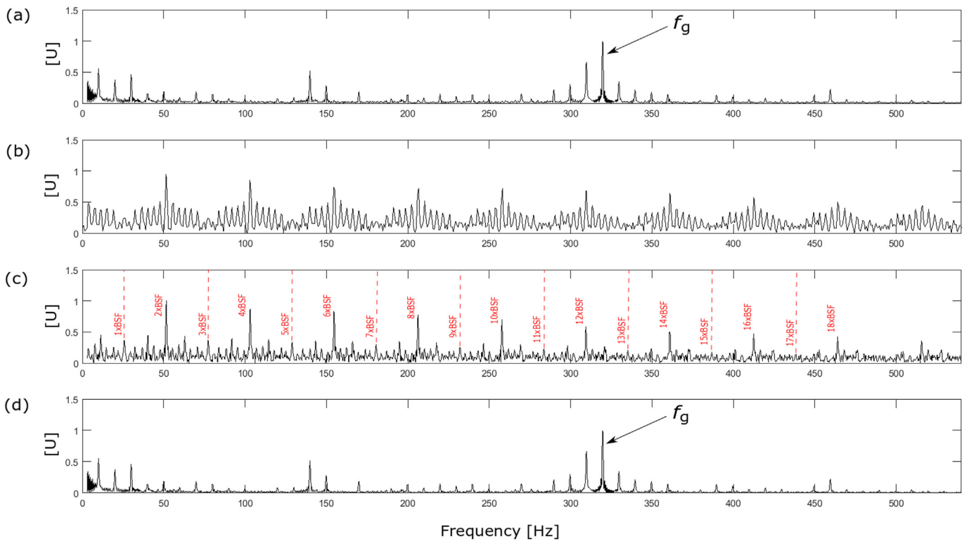
Fig. 21. Case 4. Squared Envelope Spectrum of (a) the vibration waveform: S_y^{SES}(\alpha) , (b) the band-pass filtered signal returned by the fast kurtogram, (c) the filtered time signal: S_x^{SES}(\alpha) and (d) the noise (residual) signal: S_r^{SES}(\alpha) .
