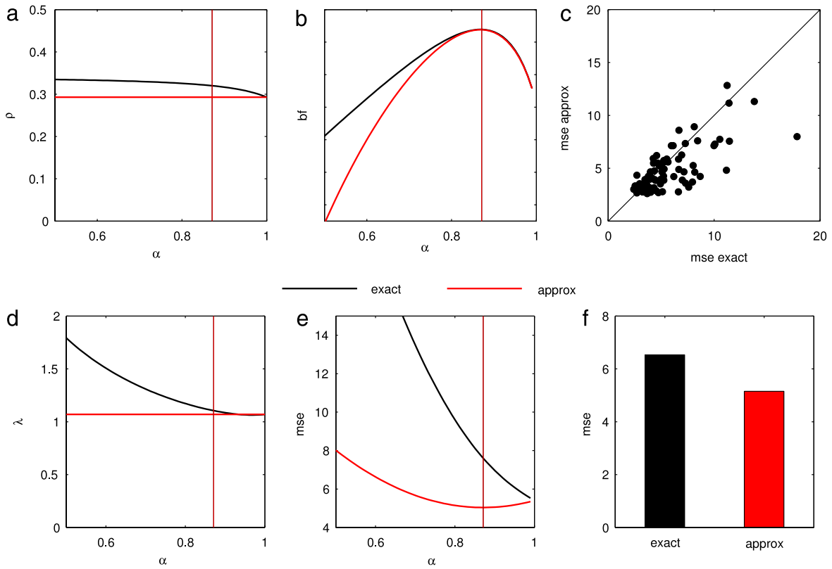
Fig. 3. Plots were obtained in situation B2, with p = 100 and n = 20 , based on one or 100 simulations. (a) Plot of the exact and approximated estimators of \rho as a function of \alpha : exact estimator \rho^* = \operatorname{argmax}_{\rho} \ell(\alpha, \lambda^*, \rho) (dark line) and approximated estimator \tilde{\rho}^* = \operatorname{argmax}_{\rho} \ell(1, \tilde{\lambda}^*, \rho) (red line). (d) Same for the exact estimator \lambda^* = \operatorname{argmax}_{\lambda} \ell(\alpha, \lambda, \rho^*) (dark line) and approximated estimator \tilde{\lambda}^* = \operatorname{argmax}_{\lambda} \ell(1, \lambda, \tilde{\rho}^*) (red line). (b) Same for \ell(\alpha, \lambda^*, \rho^*) (dark line) and \ell(1, \tilde{\lambda}^*, \tilde{\rho}^*) (red line). (e) Same for the mse \|\hat{\Sigma}^* - \Sigma\|^2 (dark line) and \|\tilde{\Sigma}^* - \Sigma\|^2 (red line). (c) Scatterplot of the mse of the exact and approximated estimators for 100 simulations. (f) Average mse of the exact and approximated estimators over 100 simulations. (For interpretation of the references to color in this figure legend, the reader is referred to the web version of this article.)
