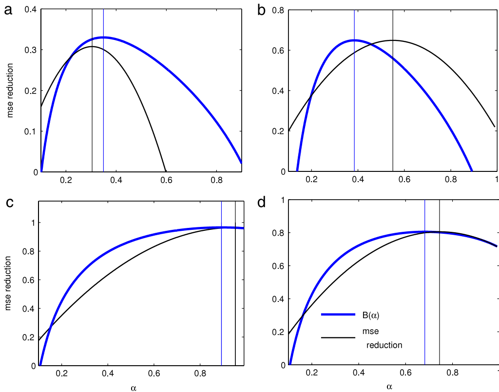
Fig. 2. Function \ell(\alpha, \mathbf{I}) (thick blue line) and % reduction in the squared estimation error \|(1 - \alpha)\mathbf{S} + \alpha\mathbf{I} - \Sigma\|^2 (light dark line) for \alpha \in [0, 1] in four different situations. (a): p = 200, n = 180 . (b): p = 20, n = 10 . (c): p = 20, n = 15 . (d): p = 20, n = 15 . The vertical lines indicate the values of \alpha maximizing \ell(\alpha, \mathbf{I}) (light blue line) and % reduction in squared estimation error (light dark line). (For interpretation of the references to color in this figure legend, the reader is referred to the web version of this article.)
