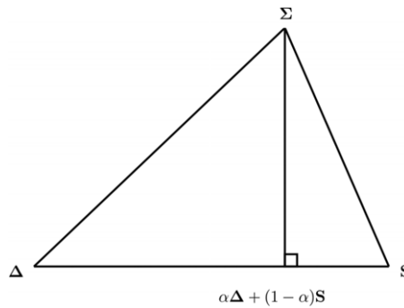
Fig. 1. After [16]. Geometric interpretation of the oracle linear shrinkage estimator as the orthogonal projection of \Sigma onto segment [S, \Delta] . Orthogonality among symmetric matrices is here defined by the inner product associated with the Frobenius norm.
