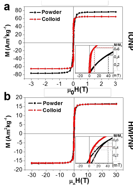
Figure 2. Magnetic hysteresis curves at 300 K of (a) IONP and (b) HMPNP. The insets present the normalized curves in which dash lines have been included as eye-guides. Both samples were measured as a powder (black) and as a colloidal suspension (red).
