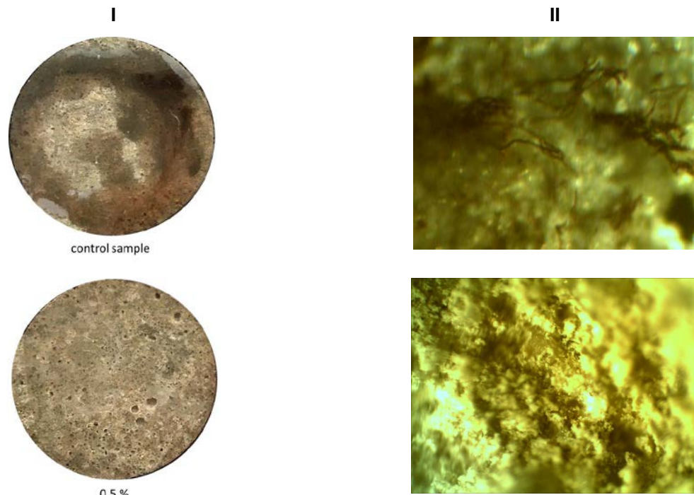
Figure 6. Antifungal effect of hardened cement-sand mortar (diameter 5 cm) with different glutardialdehyde content I – general view; II – shooting with a biological microscope (× 60 times).
