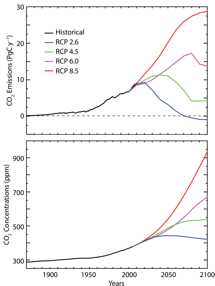
Figure 2. Carbon dioxide emissions trajectories and atmospheric CO 2 concentrations from historical data (black lines) and four of the Representative Concentration Pathways (RCPs) for the twenty-first century (colored lines) used in the most recent round of international coupled model intercomparison studies (van Vuuren et al., 2011). The RCPs span a wide range of different economic and social pathways over the twenty-first century.
