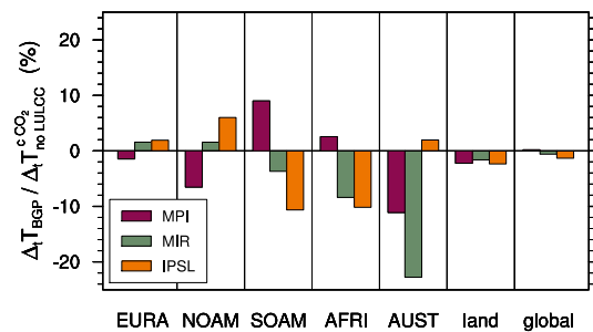
Figure 2. Relative changes in near-surface temperature: comparison of \Delta_t T_{\text{BGP}} relative to \Delta_t T_{\text{no LULCC}}^{c\text{CO}_2} (L1A simulation), that is the BGP impacts of LULCC compared to the impacts of anthropogenic carbon emissions (both fossil-fuel and LULCC) on near-surface temperature (in %). Depicted are mean 2071–2100 values minus the 2006 state (indicated by “ \Delta_t ”). Positive (negative) values indicate that BGP effects ( \Delta_t T_{\text{BGP}} ) enhance (dampen) the change caused by LULCC and other anthropogenic emissions. Analysis is done for the following regions: Eurasia (EURA), North America (NOAM), South America (SOAM), Africa (AFRI), Australia (AUST), land (land area excluding ice sheets) and global (total area on earth). A list of exact values can be found in Table S2 in the Supplement.
