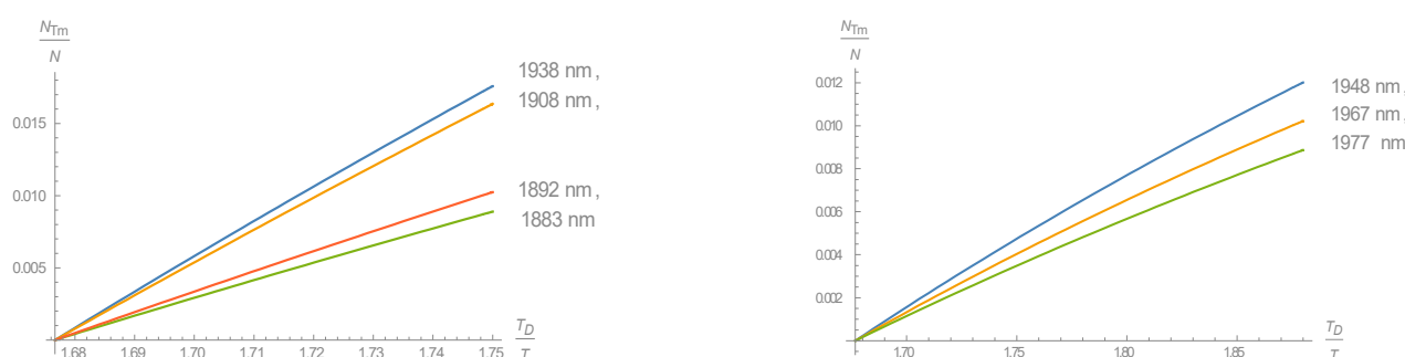
Figure 3. Concentration dependences of the cooling temperature at the excitation intensity F_p = 5 \times 10^{21} \text{ cm}^{-2} \text{ s}^{-1} at wavelengths leading to the most efficient cooling.
