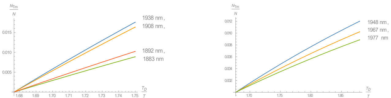
Figure 3. Concentration dependences of the cooling temperature at the excitation intensity F_p = 5 \times 10^{21} \text{ cm}^{-2}\text{s}^{-1} at wavelengths leading to the most efficient cooling.
