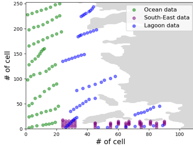
Figure 11: Position of the data for the assimilation with grouped data.
