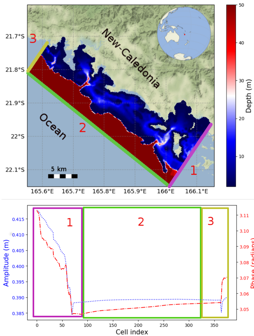
Figure 1: The upper image shows the Ouano lagoon between the ocean and the island of New-Caledonia, with the location of New-Caledonia given by the red dot in the world-map insert. We give the bathymetry of the lagoon and of the nearby ocean that we used in the model. Some water areas of the lagoon do not have bathymetry values on the map because they are very shallow reef or mangrove and we have not considered them here. The different boundaries used in the model are indicated by a colour-scale. Depths over 50 meters are found outside the lagoon. In the lower graphic, we present the boundary conditions for the amplitude and phase of the M2 tide. The colour rectangles indicate the position of the different boundaries.
