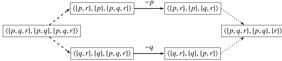
Fig. 2. Illustration of an execution of -p||-q at the model \langle\{p, q, r\}, \{p, q\}, \{p, q, r\}\rangle .
