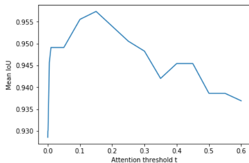
Fig. 1. Mean IoU between Attention and ground truth explanations in test set, for varying Attention threshold t . Words with Attention greater or equal to t are kept as explanation. First point is at 10^{-4} .
