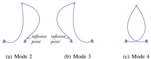
Fig. 10. The leg's buckling modes corresponding to Zones 2 and 3 in the active joint space.
