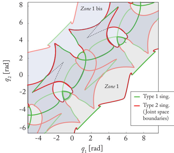
Fig. 11. Active joint space of the RFRFR robot with some unrepresented zones from Fig. 9: Zone 1 bis corresponds to Zone 1 rotated from 180^\circ deg. and translated from \pi .
