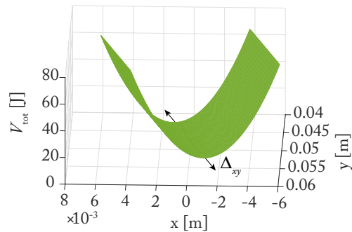
(b) Robot potential energy in the neighborhood of the configuration
