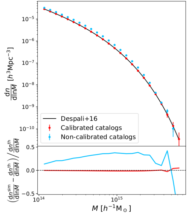
Fig. 1. Halo mass function for the mass calibration of the PINOCCHIO catalogs. Top panel: comparison between the mass function from the calibrated (red) and non-calibrated (blue) light cones, averaged over the 1000 catalogs, in the redshift bin z = 0.1 – 0.2 . Error bars represent the standard error on the mean. The black line is the D16 mass function. Bottom panel: relative difference between the mass function from simulations and that of D16.
