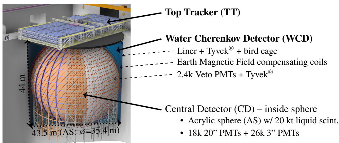
Figure 1: The JUNO detector. The Veto System components are shown in bold.
