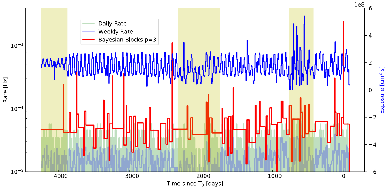
Extended Data Fig. 3. Bayesian Blocks representation of the arrival times of the \gamma rays with the prior parameter p=3 . Light green and light blue are the daily and weekly count rates, while the blue curve shows the weekly-averaged exposure (between 100 MeV and 300 GeV, assuming a power-law photon index of -2 ) for a 1^\circ -radius ROI in the direction of Sculptor for the entire time of the mission. The three yellow bands highlight three characteristic observing profiles: 35^\circ rocking angle, at the beginning of the mission, an observation strategy favoring the Galactic Center region, in the middle, and, lastly, the period between the start of the solar drive anomaly and the implementation of a reoptimized survey strategy.
