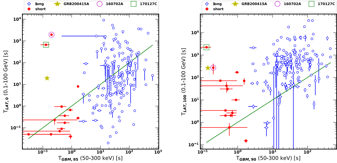
Extended Data Fig. 4. Left: onset times ( T_{\text{LAT},0} ) in the 100 MeV–100 GeV band vs. the end of the GRB as detected by GBM in the 50–300 keV energy range ( T_{\text{GBM},95} ). Right: Durations ( T_{\text{LAT},100} ) calculated in the 100 MeV–100 GeV energy range vs. the same quantities calculated in the 50–300 keV energy range ( T_{\text{GBM},90} ). The solid line denotes where the two values are equal. Empty Blue and filled red circles represent long and short GRBs, respectively (data from 2FLGC 3 ). GRB 200415A is added and marked with a yellow star. The two SGRBs 160702A and GRB 170127C from 2FLGC, which exhibit similar durations, are highlighted with a magenta circle and green square, respectively.
