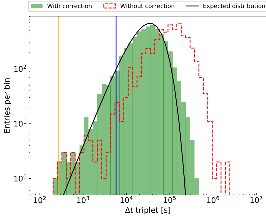
Extended Data Fig. 2. Distribution of the time intervals \Delta t for triplets formed by three consecutive photons with (green) and without (dashed red) taking into account the correction for the effects of the LAT orbit and FOV. The expected distribution in case of independent events is represented as a solid black line. The vertical line in blue shows the period of the Fermi orbit (5790 s), while the orange vertical line indicates \Delta t = 264.87 s corresponding to the photon triplet detected by the LAT after GBM detected emission from GRB 200415A.
