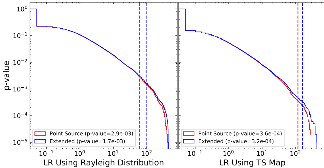
Extended Data Fig. 1. Likelihood Ratio (LR) values for 10^5 simulated ROIs. Left: using the standard Rayleigh formula, right: using the TS map to compute the probability. The red distributions correspond to the point source hypothesis, while the blue distributions take into account of the galaxy extension. The step in the distributions at low LR is due to many low-LR trials occupying the first bin. The value of the LRs associated with the Sculptor galaxy are highlighted by red and blue vertical dashed lines for the two cases.
