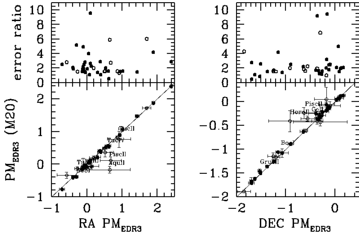
Figure A1. Comparison of proper motions (left: RA, right: DEC) of Table 1 with those calculated by McConnachie & Venn (2020). Few dwarf galaxies names are indicated, pointing out to dwarf galaxies for which the two measurements are discrepant at > 1 \sigma level. The top panels indicate the ratio of error from this paper to that tabulated by McConnachie & Venn (2020) both extracted from Gaia EDR3. Notice that the error on PM RA of Fornax is so small ( 1 \mu\text{s yr}^{-1} ) in McConnachie & Venn (2020) that it leads to a ratio in excess of 20 (not shown in the Figure).
