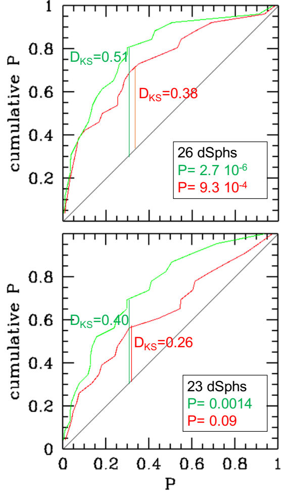
Figure 3. Cumulative distribution of time to reach the pericenter divided by the time taken from pericenter to min(apocenter, 300 kpc). The black solid line shows the null hypothesis, i.e., dwarf galaxies have location randomly distributed from pericenter to min(apocenter, 300 kpc). Green and red lines represent the PNFW model ( M_{tot} = 8.1 \times 10^{11} M_{\odot} , see also Eilers et al. 2019, and PE_{HM} the most massive mass able to fit the MW rotation curve ( M_{tot} = 15 \times 10^{11} M_{\odot} , see Jiao et al. 2021), respectively. D_{max} values and associated probabilities of the Kolmogorov Smirnov tests are given in the Figures, top and bottom panels representing the 90.5 (dubbed as small volume) and the 181 kpc (dubbed as large volume) distance slices of Drlica-Wagner et al. 2020, respectively.
