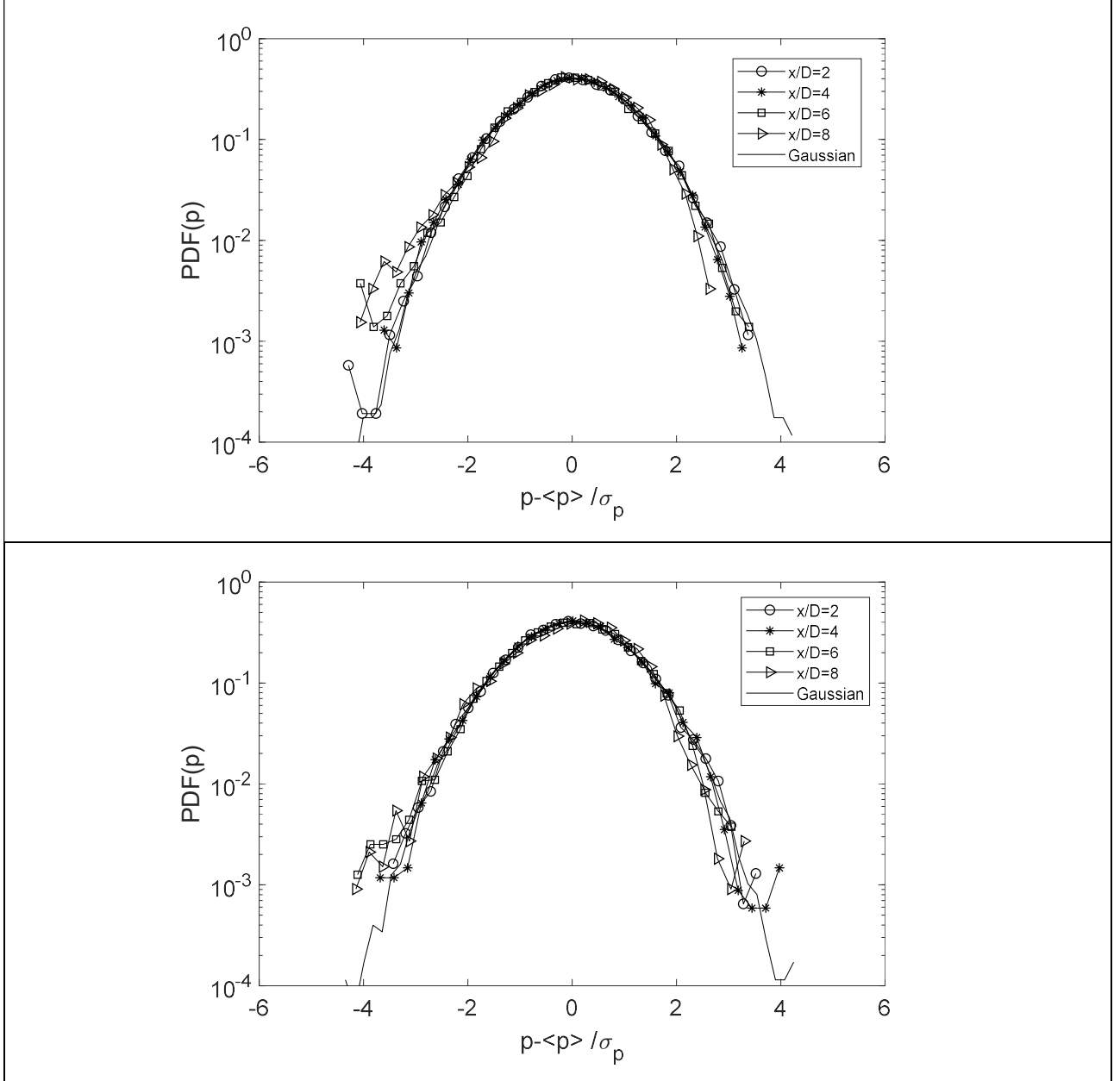
Figure 9: PDF of the mode-0 pressure fluctuations at the low (top) and high (bottom) Re computed at r/D=1 for different axial positions. The solid line is the PDF of a reference Gaussian signal obtained by a random numbers generator.
