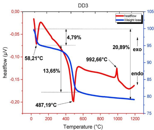
Figure 7 : TDA/TG curves of Algerian kaolin heated up to 1200°C with rate of 10 °C/min: (A) DD1, (B) DD2, (C) DD3.
