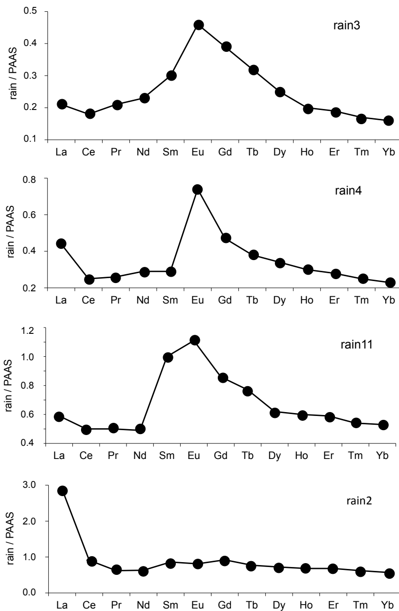
Figure 5: Some characteristic rare-earth elemental distribution patterns of rain solutes relative to the PAAS reference.
