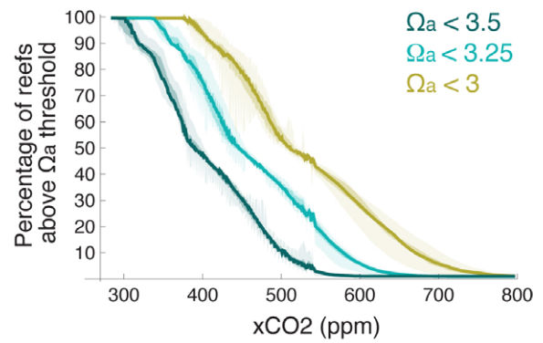
Figure 3. Percentage of coral reefs surrounded by open ocean waters above aragonite saturation thresholds as a function of atmospheric CO_2 concentration. The ensemble median (lines), quartiles (darker shading) and range (lighter shading) are displayed for aragonite saturation thresholds ( \Omega_{a,crit} ) of 3.5, 3.25 and 3. The narrow spread across all models and emissions scenarios considered indicates that xCO_2 is a good predictor of the distribution of aragonite saturation around coral reefs.
