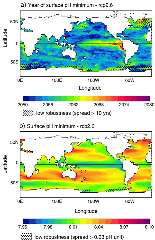
Figure 3. Model-mean pH in RCP2.6 scenario: (a) year of surface pH minimum, (b) surface pH minimum value. Stippling indicates poorer agreement, i.e., where the model spread is larger than: (Figure 3a) 10 years and (Figure 3b) 0.03 pH unit. Figure based on the six models with pH for RCP2.6 (GFDL-ESM2G, GFDL-ESM2M, IPSL-CM5A-LR, IPSL-CM5A-MR, MPI-ESM-MR, and NorESM1-ME).
