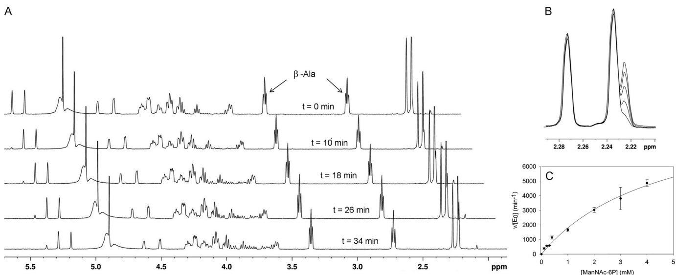
FIGURE 4. Real time ^1\text{H} NMR analysis of CpNanE activity. A, time course of ManNAc-6P (2 mM) epimerization by CpNanE in the presence of \beta -alanine (1 mM) as an internal standard was monitored. Selected regions of the spectra acquired between 0 and 34 min are shown. B, overlay of the spectral region from 2.2 to 2.3 ppm showing the disappearance of the characteristic peak for the ManNAc-6P methyl resonances versus appearance of GlcNAc-6P methyl resonance. C, initial velocities of ManNAc-6P epimerization by CpNanE in the presence of different concentrations of ManNAc-6P. A Michaelis-Menten curve was fitted using the formula: v/[E]_0 = k_{\text{cat}} [S]/(K_m + [S]) .
