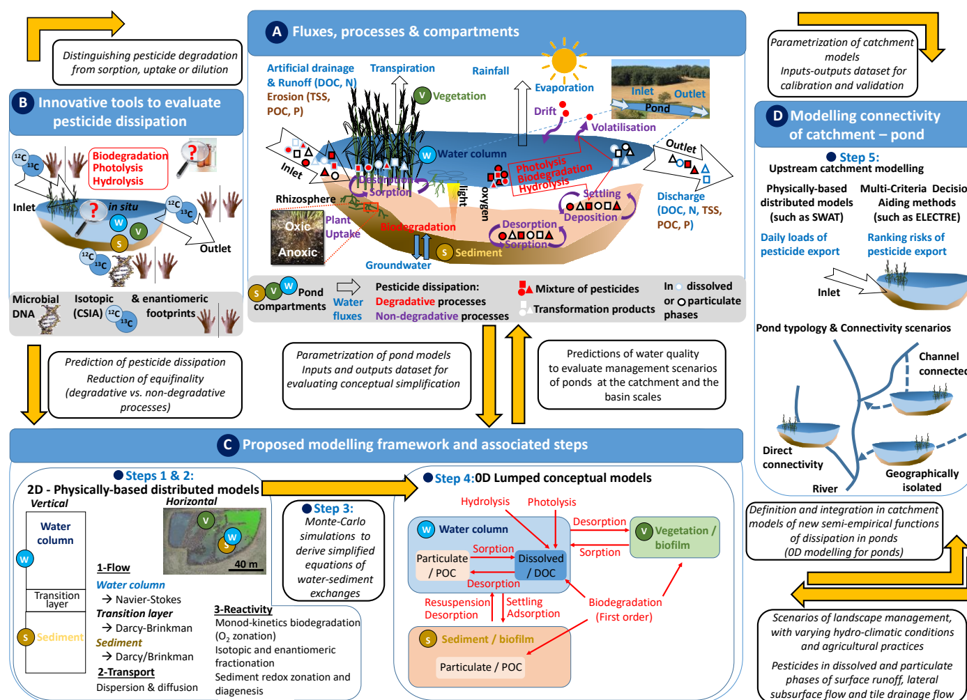
Figure 1. Evaluation and prediction of pesticide dissipation in ponds and the role of ponds at the catchment scale. (A) Fluxes, processes and compartments of ponds. (B) Innovative tools to distinguish pesticide degradative and non-degradative processes. (C) Pond modelling framework sketched in this review and associated steps. (D) Modelling the catchment–pond connectivity to integrate the cumulative effect of ponds in terms of risks of pesticides transfer and fluxes at the catchment scale and elaborate management scenarios. TSS: total suspended solids; DOC: dissolved organic carbon; N: nitrogen; P: phosphorus; POC: particulate organic carbon.
