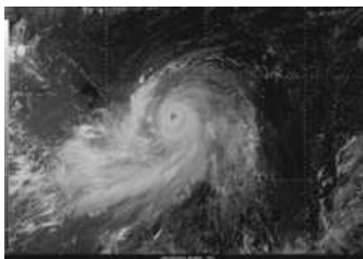
Meteorologic dynamic models allow a typhoon evolution to be predicted over 48h.
