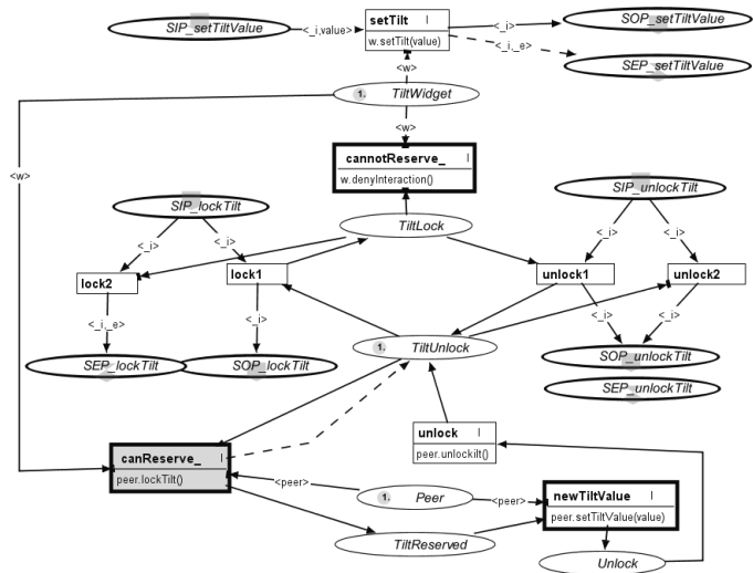
Fig. 7. Excerpt of the ND application model
