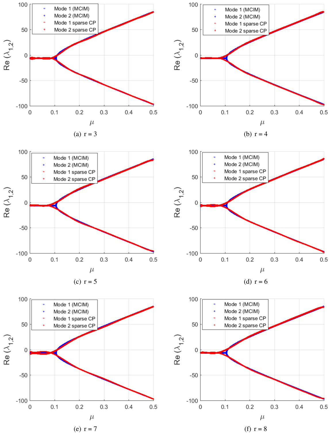
Figure 4: Real parts of mode 1 and 2 using MCIM and Sparse PC
